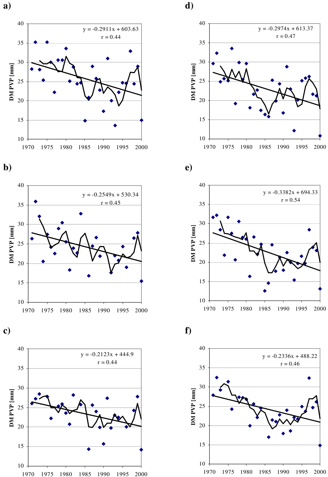
Fig. 3 Long-term tendency and 5-year moving average of De Martonne annual aridity index for the Planning Regions: a) Northwestern; b) North Central; c) Northeastern; d) Southwestern; e) South Central; f) Southeastern
