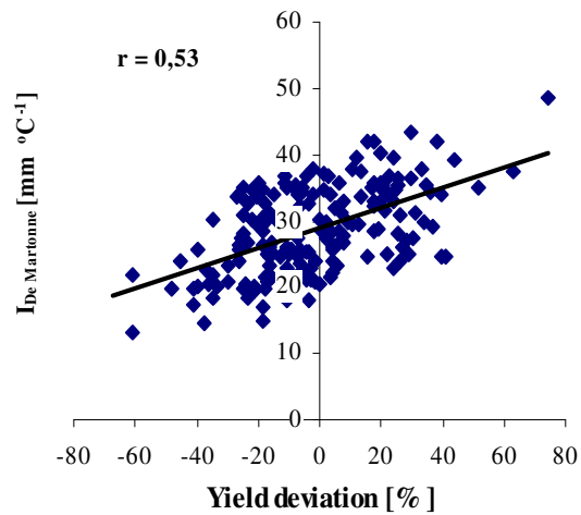
Fig. 7 Relation between winter wheat yield deviation from the average 30-year one and De Martonne aridity index
