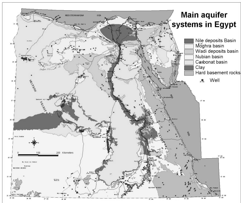
Figure (2): Surface Distribution of Aquifer System
