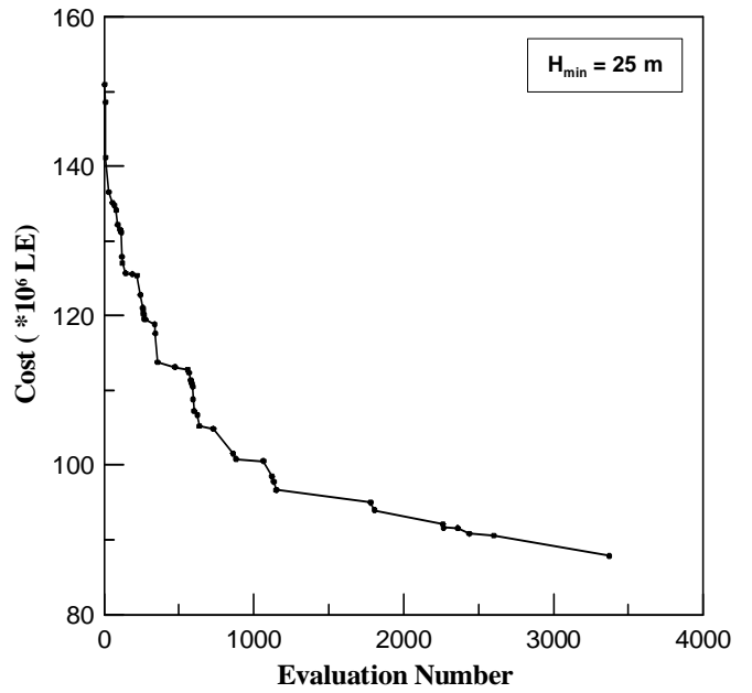
Figure 6. Cost evolution for H_{min} = 25 m
