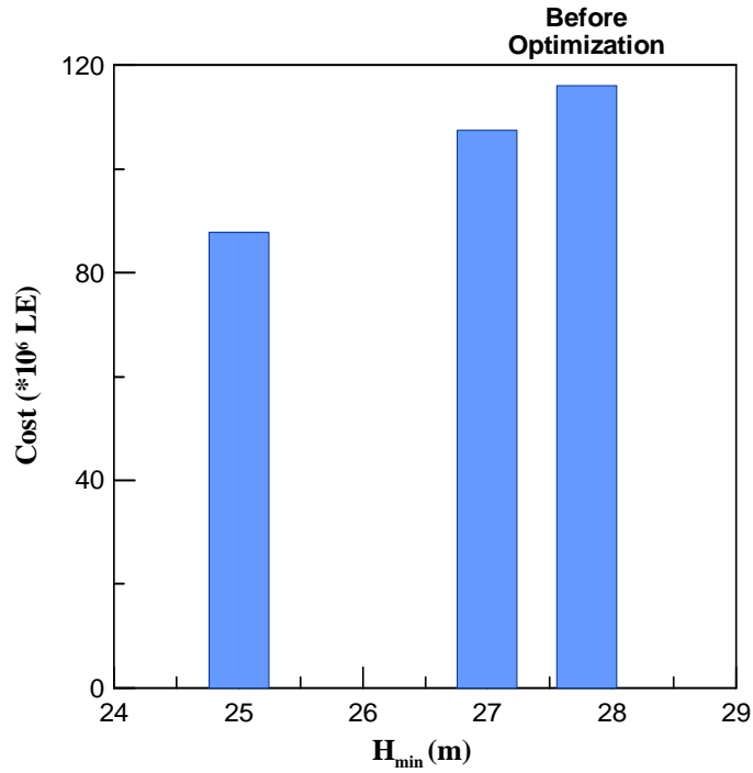
Figure 4. Comparison between costs before and after optimization for H_{min} = 25 m and H_{min} = 27 m
